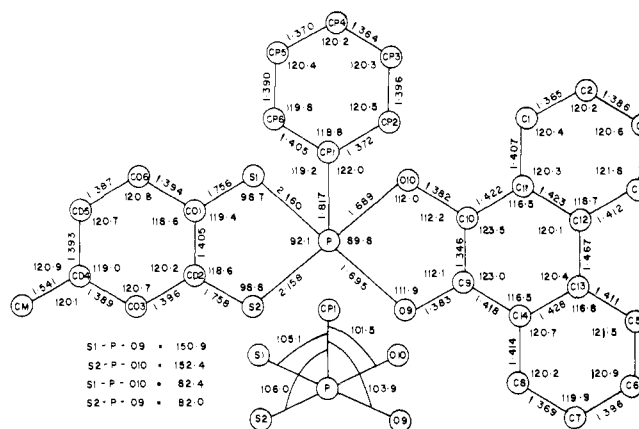
Figure 2. Selected bond lengths in Å and angles in degrees for (\text{CH}_3\text{C}_6\text{H}_3\text{S}_2)(\text{C}_{14}\text{H}_8\text{O}_2)\text{PPh} (III).
