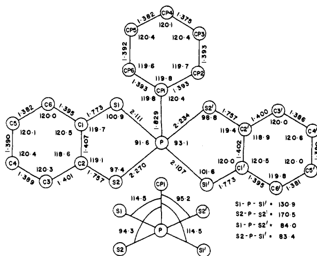
Figure 6. Selected bond lengths in ångströms and angles in degrees for (\text{C}_6\text{H}_4\text{S}_2)_2\text{PPh} (V).
