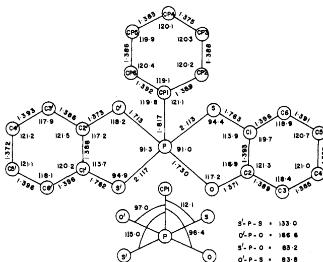
Figure 4. Selected bond lengths in ångstroms and angles in degrees for (\text{C}_6\text{H}_4\text{OS})_2\text{PPh} (IV).
